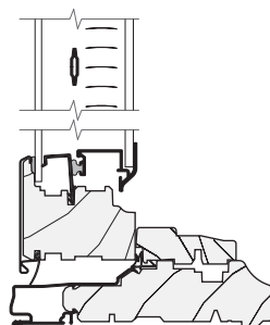
Designer Series Double-Pane Glazing, with Removable Between-Glass Grilles and Slimshade Blinds
