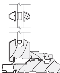
Architect Series with 7/8" Regular Integral Light Technology Grilles
