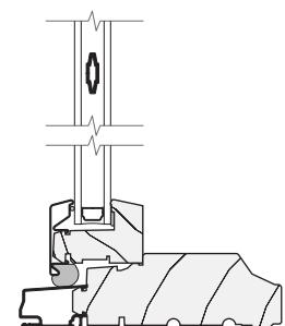
Pella® ProLine with Grilles-Between-the-Glass
