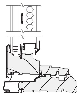
Designer Series Triple-Pane Glazing, with Removable Between-Glass Grilles and Cellular Fabric Shades
