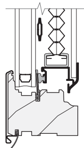
Grilles and Cellular Fabric Shades
