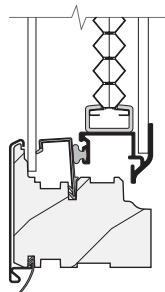
Cellular Fabric Shades
