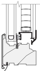
Raise and Lower or Tilt only Blinds
